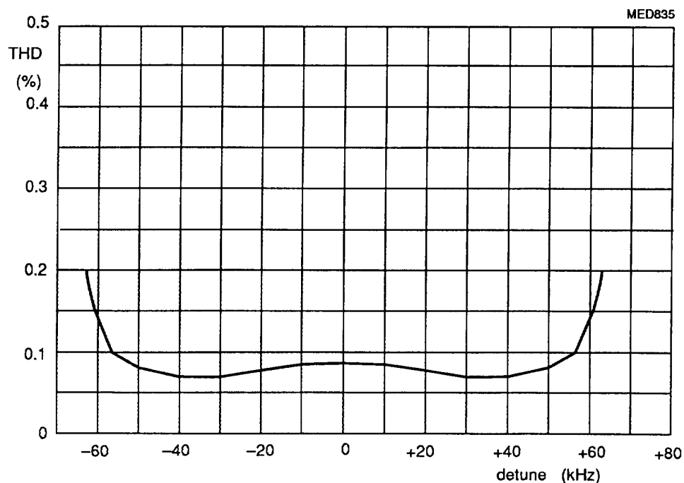
Fig.17 Total harmonic distortion dependent on detuning at FM-MUTE-ON; deviation \pm 75 \text{ kHz} ; f_m = 1 \text{ kHz} ; V_{\text{ilF}} = 10 \text{ mV} .
